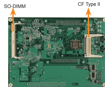
Solder Side
